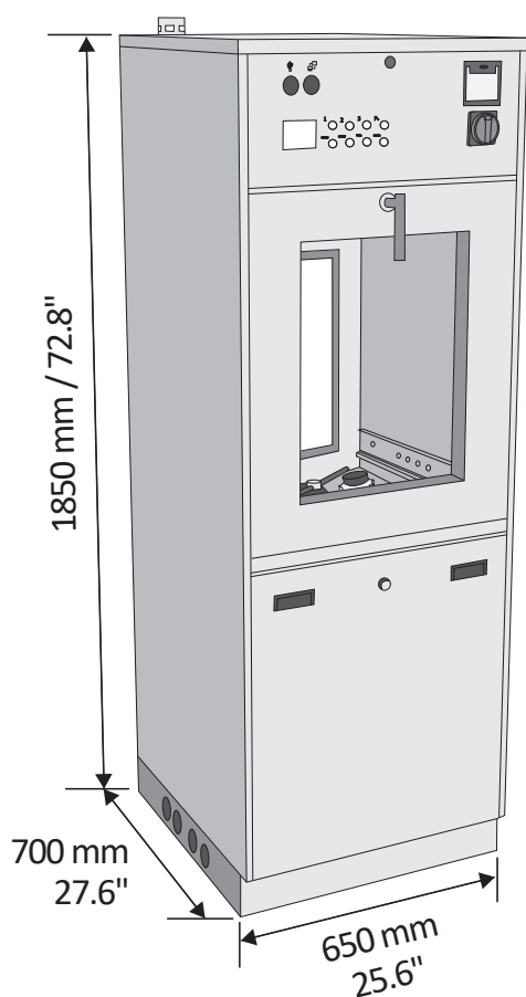
AWD655-10D Pass-through doors without boiler
