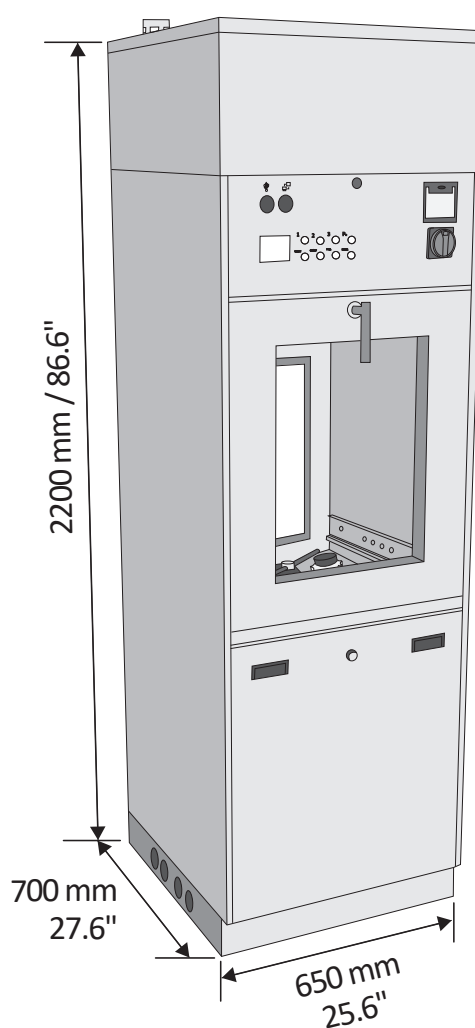
AWD655-10D-SC AWD655-10D-2SC Pass-through doors with boiler
