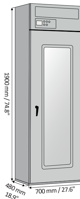
DCI-70 Single Door
